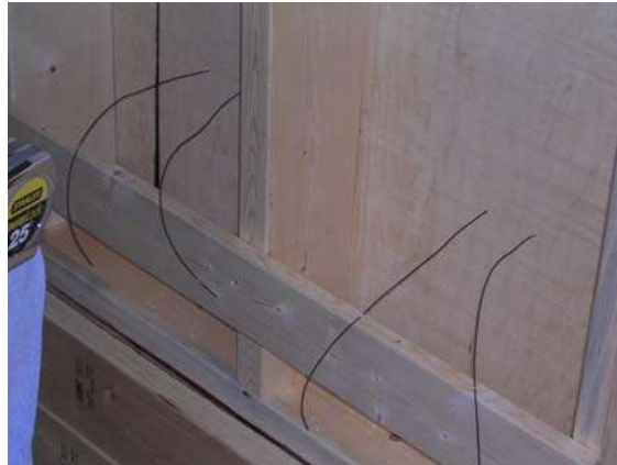
Figure 4: Plywood Layer sensor wires, rear view
